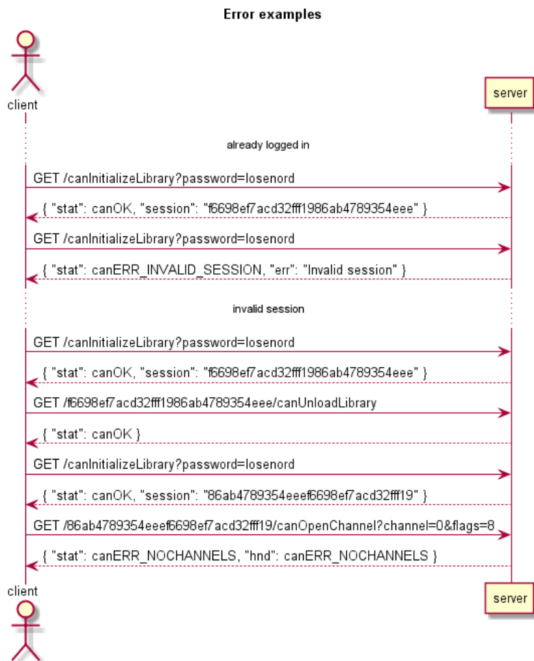
Figure 8: Error examples
